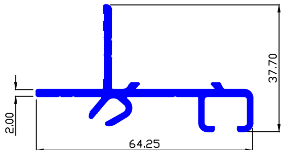
MAAN SEC.-89473 0.711 Kg/Mtr.
