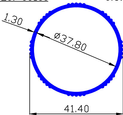
MAAN SEC.-90199 0.478 Kg/Mtr.
