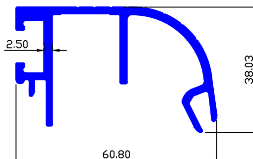
MAAN SEC.-89592 1.029 Kg/Mtr.
