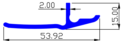
MAAN SEC.-90242 0.385 Kg/Mtr.
