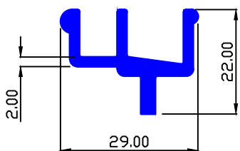
MAAN SEC.-89586 0.450 Kg/Mtr.
