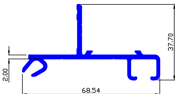
MAAN SEC.-89591 0.717 Kg/Mtr.
