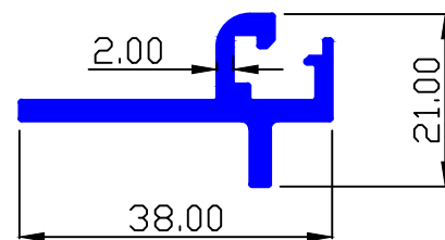
MAAN SEC.-90241 0.449 Kg/Mtr.
