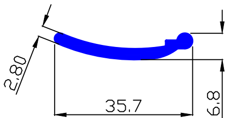
MAAN SEC.-90227 0.281 Kg/Mtr.
