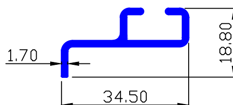
MAAN SEC.-90243 0.305 Kg/Mtr.
