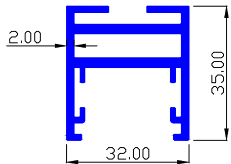
MAAN SEC.-91063 0.298 Kg/Mtr.
