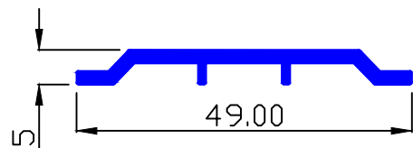
MAAN SEC.-91063 0.298 Kg/Mtr.
