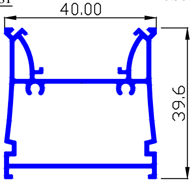
MAAN SEC.-90281 0.588 Kg/Mtr.
