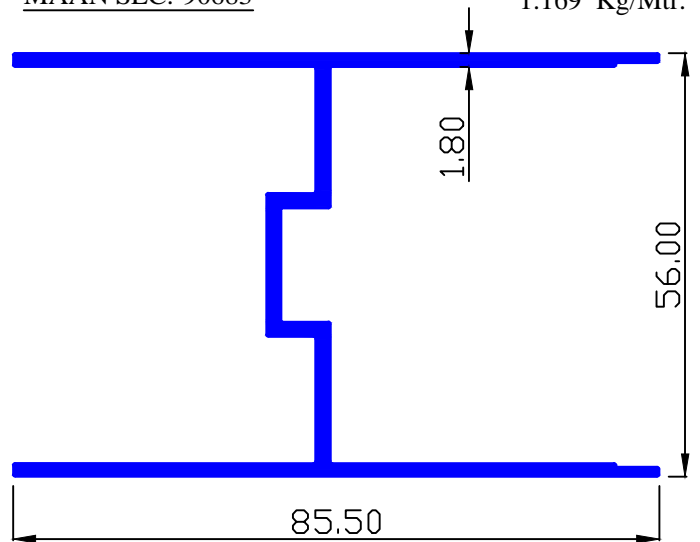
MAAN SEC.-90683 1.169 Kg/Mtr.
