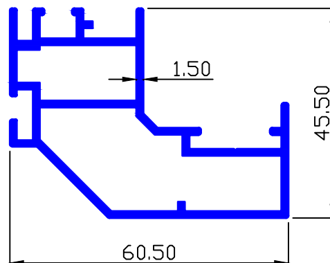
MAAN SEC.-7014 1.067 Kg/Mtr.
