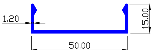
MAAN SEC.-89489 0.315 Kg/Mtr.
