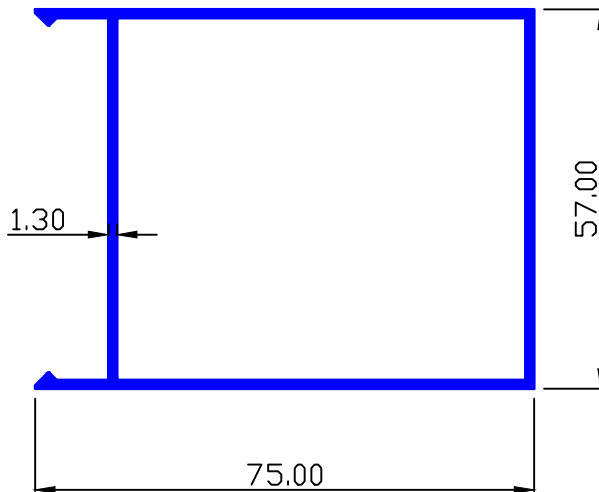
MAAN SEC.-89489 0.315 Kg/Mtr.
