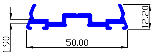
MAAN SEC.-89494 0.413 Kg/Mtr.
