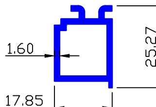
MAAN SEC.-89158 0.353 Kg/Mtr.
