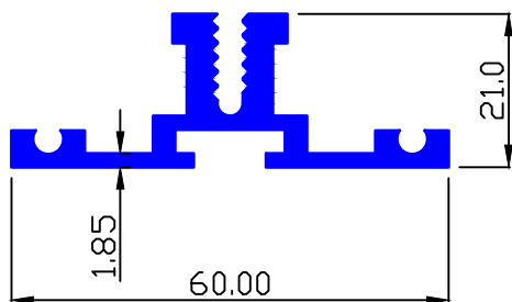
MAAN SEC.-6843 0.859 Kg/Mtr.
