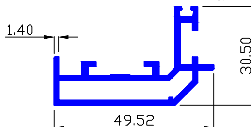
MAAN SEC.-89159 0.673 Kg/Mtr.
