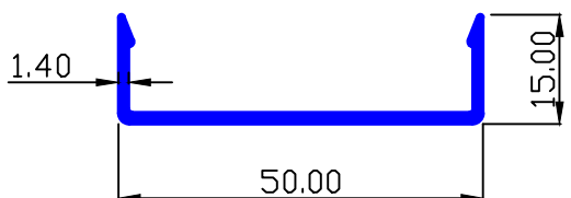
MAAN SEC.-89493 0.323 Kg/Mtr.
