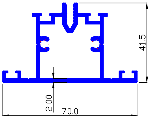
MAAN SEC.-7013 1.179 Kg/Mtr.
