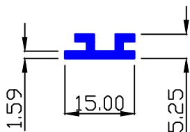
MAAN SEC.-89148 0.120 Kg/Mtr.
