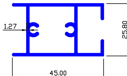
MAAN SEC.-8098 0.590 Kg/Mtr.
