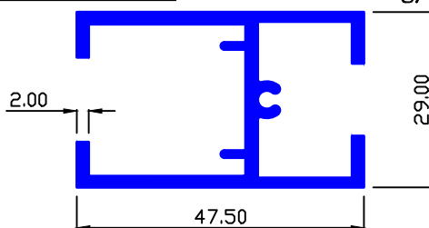
MAAN SEC.-89406 0.799 Kg/Mtr.
