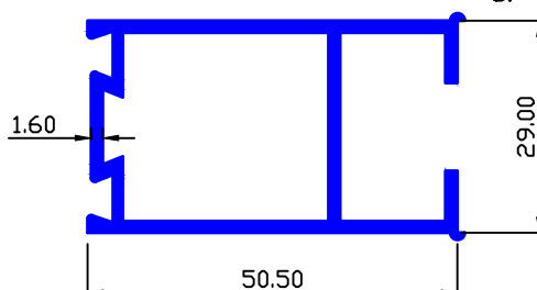
MAAN SEC.-89400 0.767 Kg/Mtr.
