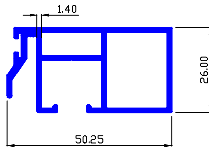
MAAN SEC.-90143 0.769 Kg/Mtr.
