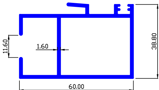
MAAN SEC.-8050 0.972 Kg/Mtr.
