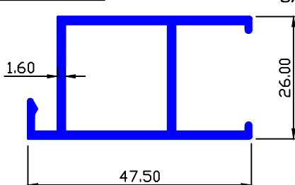
MAAN SEC.-89402 0.622 Kg/Mtr.
