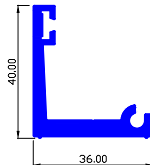
MAAN SEC.-90148 0.861 Kg/Mtr.
