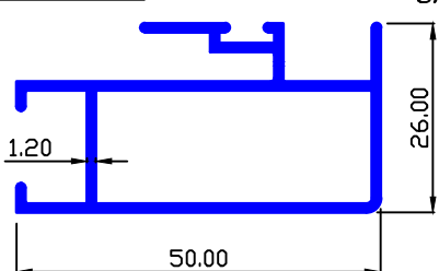
MAAN SEC.-89391 0.568 Kg/Mtr.
