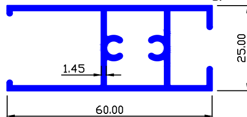
MAAN SEC.-89387 0.784 Kg/Mtr.
