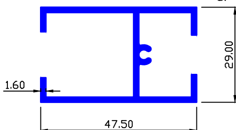
MAAN SEC.-89397 0.663 Kg/Mtr.
