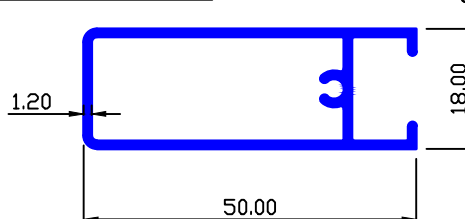
MAAN SEC.-89392 0.463 Kg/Mtr.
