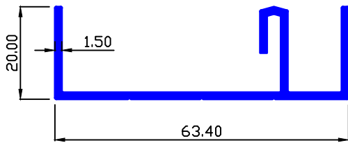
MAAN SEC.-90156 0.529 Kg/Mtr.
