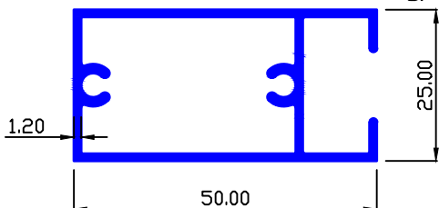
MAAN SEC.-89386 0.593 Kg/Mtr.
